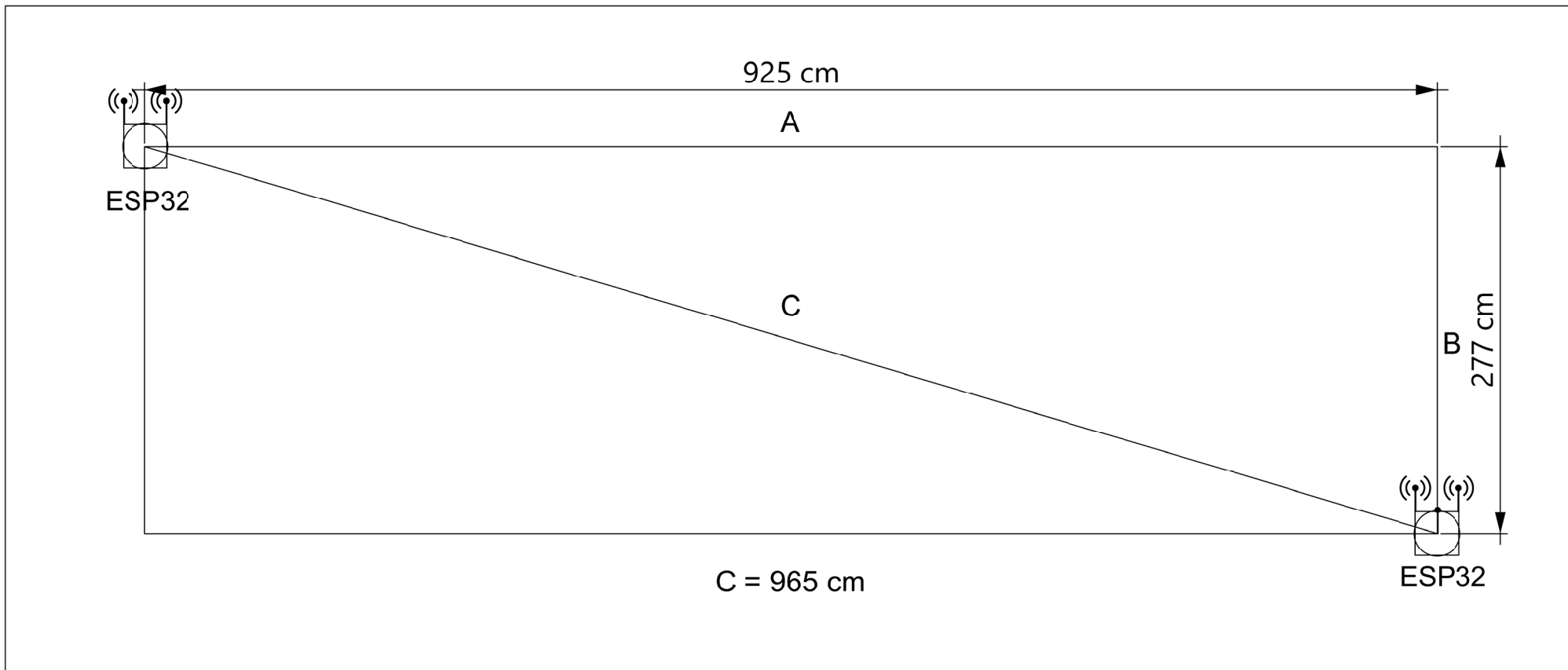
Figure: WiFi Sensing prototyping layout
